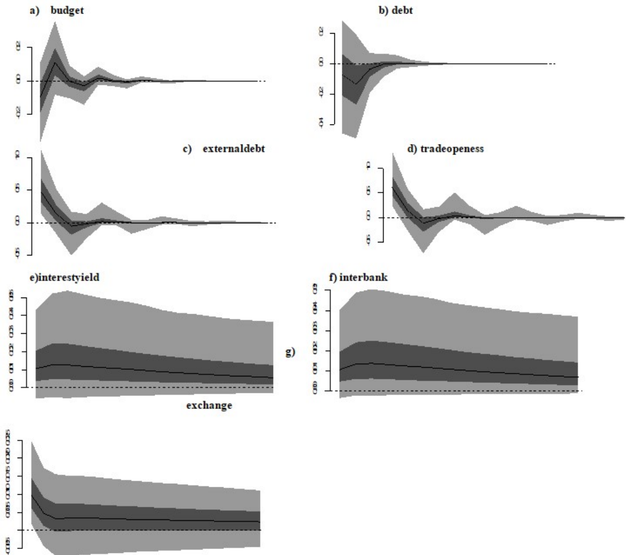
Figure 1. Impulse-Response Functions
